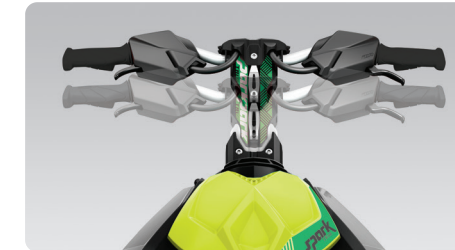
Handlebar with adjustable riser A telescopic steering system that optimizes the experience for varying rider sizes.
